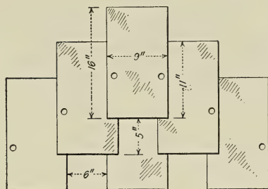
FIG. 137.—Wide-spaced Shingles.
